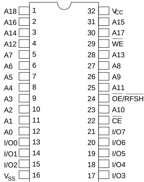
HM658512ALP/ALFP Series
